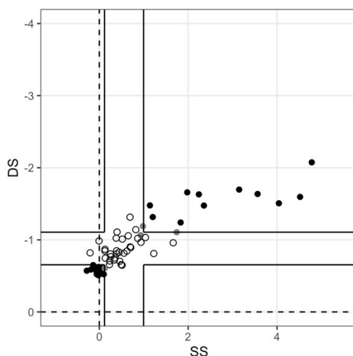
Figure 5 - Zooplot for system with LTF4 as input
