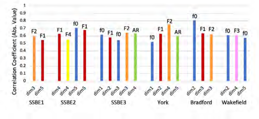
Figure 2 - Significant correlations (absolute value) between the acoustic features tested and the five pseudo-perceptual dimensions generated by the listeners’ voice similarity judgements by the MDS analysis for each speaker group, dimensions 1 to 5, labelled dim1, dim2, etc.
