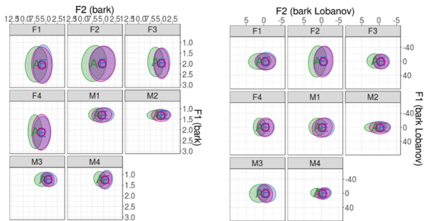
Figure 13 - Un-normalized Vs normalized vowel space for spontaneous speech
