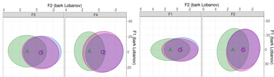
Figure 15 - Normalized distributions for the second female couple
