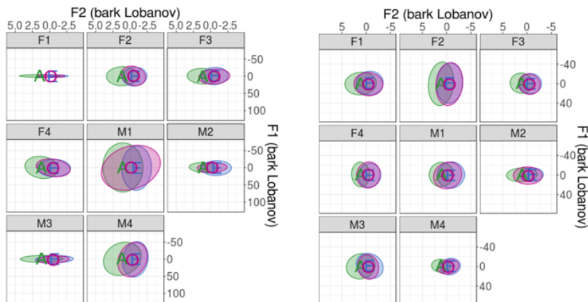
Figure 14 - Elicited Vs Spontaneous normalized vowel space
