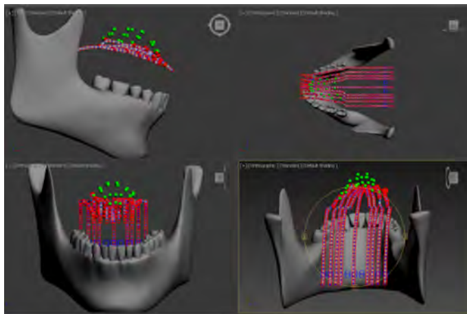
Figure 2 - Transposition of the 42 UTI fan radii into 9 chains of 42 bones each (four different visualization angles). The 9 chains are in red. Each dot of the chain represents one bone. Green dots represent the electrodes on palate surface, here provided for reference
