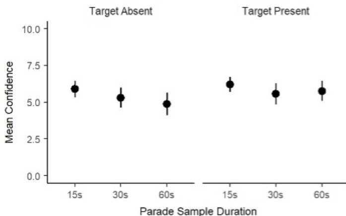
Figure 5 - Mean confidence ratings of participants in target-present and target-absent parades for 15s, 30s and 60s conditions. Error bars show 95% confidence intervals for the condition means
