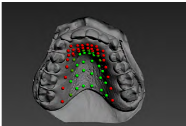
Figure 4 - The artificial palate with sensors in the 3D model. Red dots: contacted sensors. Green dots: no tongue contact
