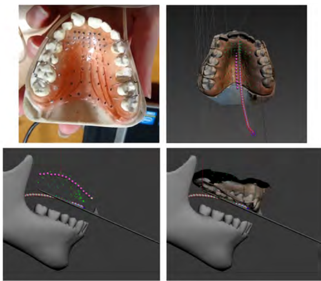
Figure 3 - Top left: the EPG artificial palate and its chalk cast. Top right: Virtual palate modeling with positioning in the midsagittal plane. Bottom left: Ultrasound trajectory of the palate. Bottom right: superposition of the artificial palate
