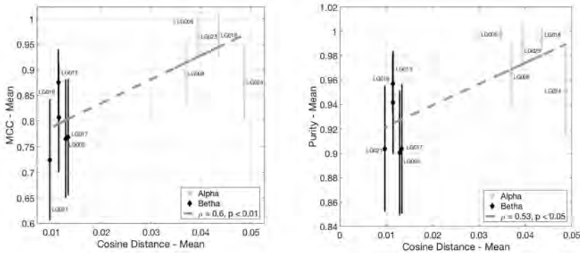
Figure 4 - Pearson correlation procedures applied to: speaker CDS and MCC means with \rho = 0.6 , p < 0.01 (Left) and speaker CDS and Purity means with \rho = 0.53 , p < 0.05 (Right). Diamonds and vertical lines represent means and standard error, respectively. Text refers to speaker identification
