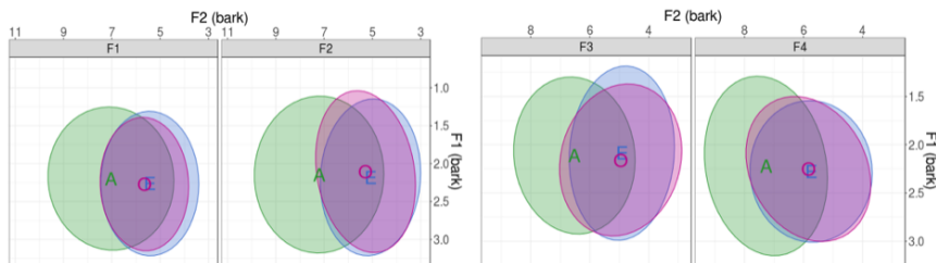
Figure 7 - Elicited speech vowel space for female pairs
