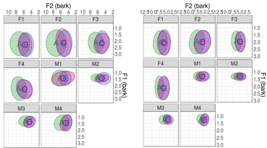
Figure 5 - Elicited and spontaneous speech for all pairs
