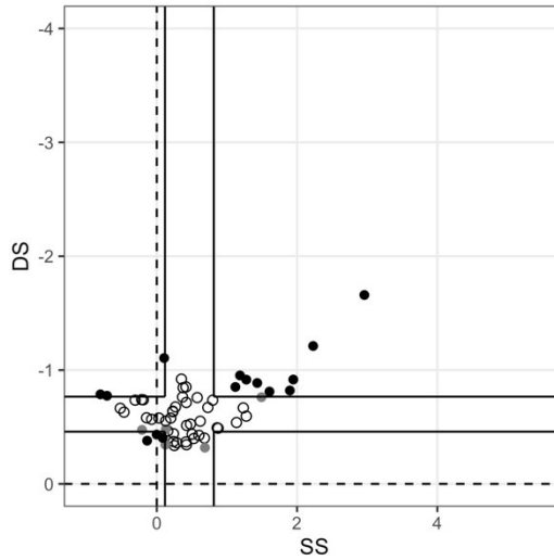
Figure 3 - Zooplot for system with LTF2 as input
