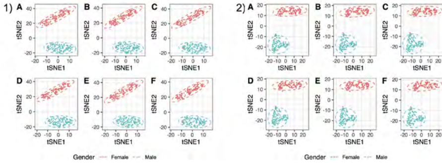
Figure 4 - t -SNE reduced two-dimensional spaces of AISHELL-1 speakers from i-vector (1) 400-dimension and x-vector (2) 512-dimension speaker embeddings
