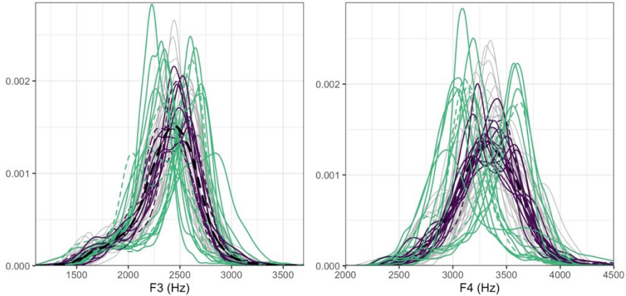
Figure 8 - Distributions of LTF3 (left) and LTF4 for all speakers, with doves in green, worms in purple and other speakers in grey (dashed coloured lines indicate near-members of animal groups; black dashed line indicates group distribution pooled from all 60 speakers)
