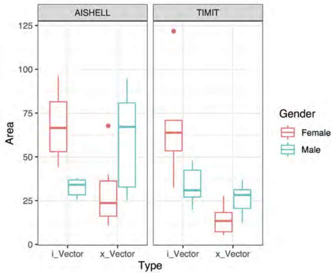
Figure 5 - Cluster area of speaker embeddings from TIMIT and AISHELL-1 datasets in the 2-dimension t -SNE space
