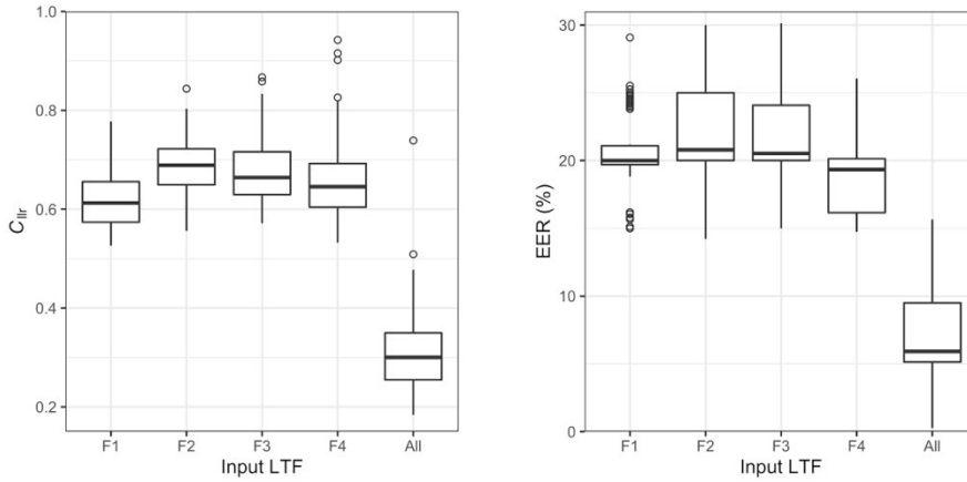
Figure 1 - Boxplots of C_{llr} (left) and EER (right) from system testing
