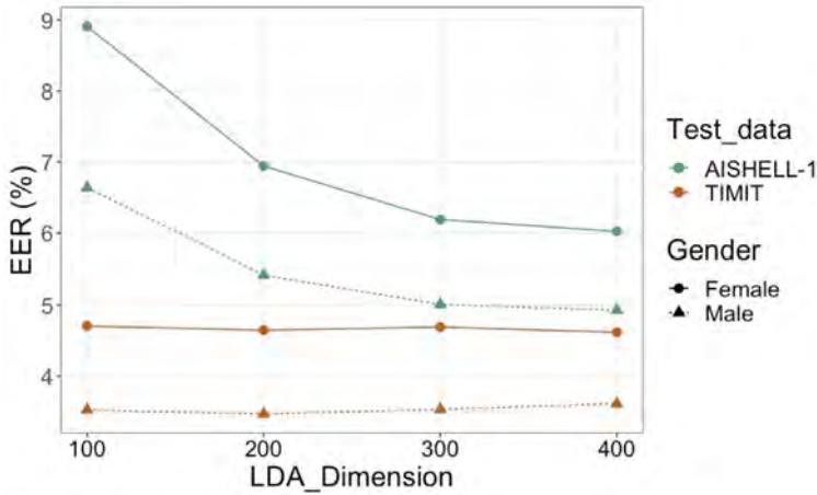
Figure 1 - The speaker recognition performance (EER%) of the i-vector system in 2 different datasets and different genders. The LDA -dimension is varied in the range of 100 to 400 with 100 step-sizes
