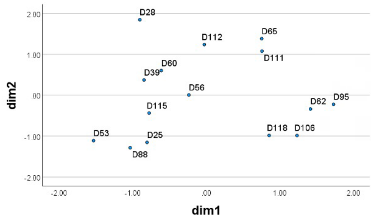
Figure 1 - Plot of the first two dimensions (of five) produced by the MDS analysis for the SSBE 1 group, showing the relative positions among the 15 speakers
