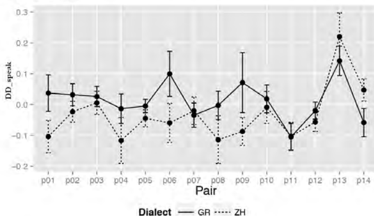
Figure 3a-b - Line chart showing the difference in distance within speaker ( DD_speak ) per dialect and pair for vowel formants (top panel, plot in Ruch, 2015), and segmental durational properties (bottom panel). Dot represents average values, whisker error bar over all target words per speaker
