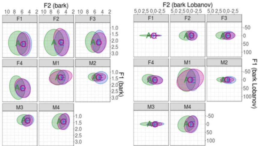
Figure 1 - Vowel space for elicited speech before and after Lobanov's normalization
