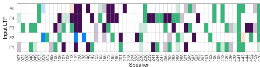
Figure 7 - Summary of speakers classified as doves (green), worms (purple), phantoms (blue) or chameleons (orange) in all systems tested (near-members of each group in lighter shade)
