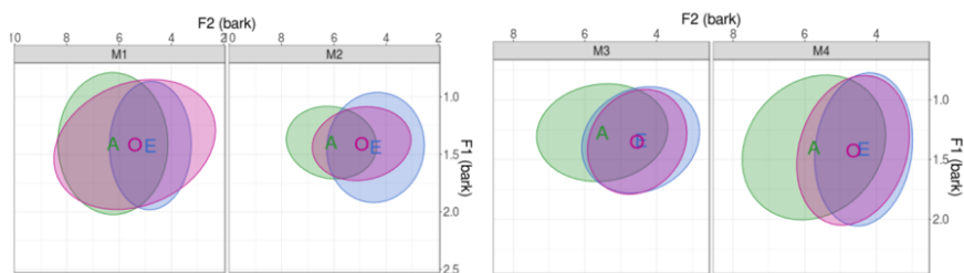
Figure 4 - Male couples' vowel space
