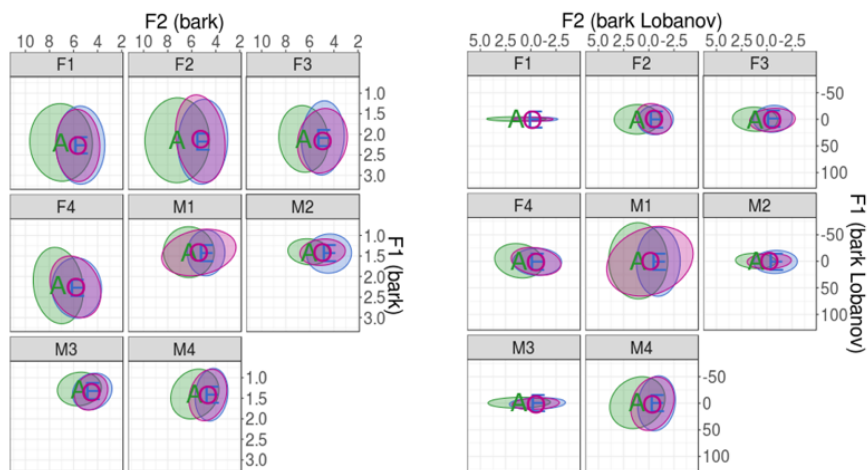
Figure 10 - Vowel space before and after Lobanov's normalization
