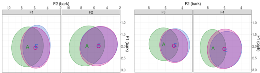
Figure 6 - Spontaneous speech vowel space for female pairs
