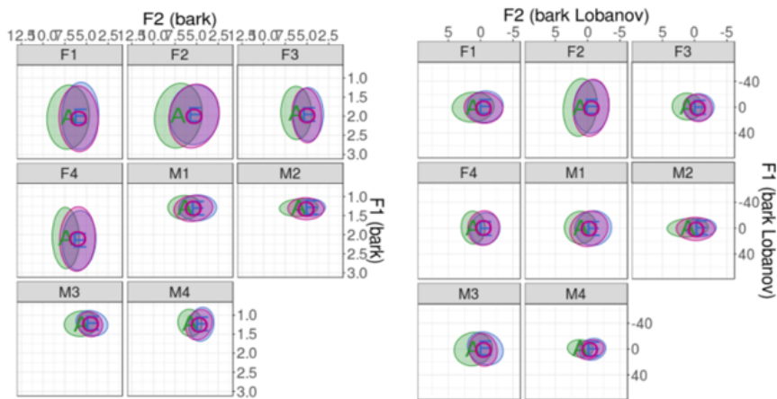
Figure 2 - Vowel space for spontaneous speech and for all speakers before and after Lobanov's normalization
