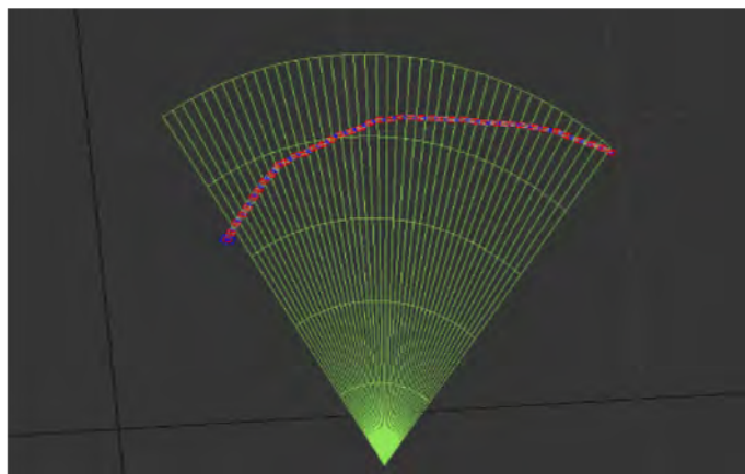
Figure 1 - Two-dimensional reconstruction of the 42 UTI fan radii and tongue spline
