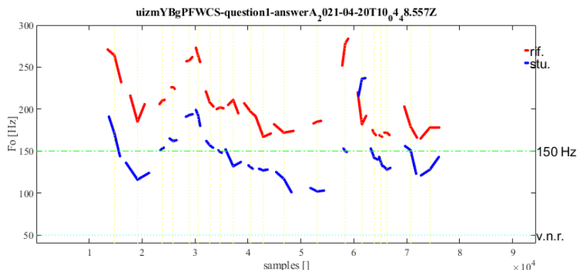
Figure 5 - Comparison of intonation curves between reference speaker (red) and user (blue) of the utterance “Scusi, ho lasciato l’orologio a casa, sa dirmi che ore sono?”
