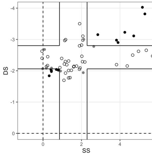
Figure 6 - Zooplot for system with all four LTFs as input
