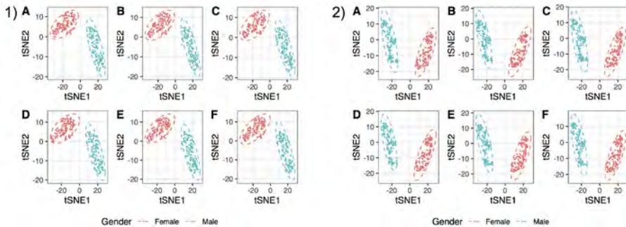
Figure 3 - t-SNE reduced two-dimensional spaces of TIMIT speakers from i-vector (1) 400-dimension and x-vector (2) 512-dimension speaker embeddings
