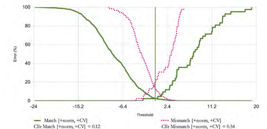
Figure 3 - Tippett plot: normalised and calibrated scores using cross validation calibration [+norm, +CV] in the match condition [voice message] (solid green) and the mismatch condition [voice message – telephone] (dotted pink)
