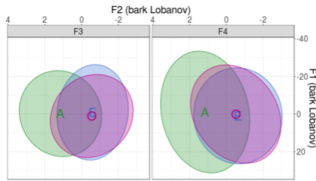
Figure 12 - Comparison of normalized distributions for the second female couple
