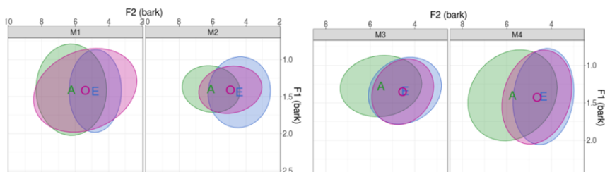
Figure 9 - Elicited speech vowel space for male couples
