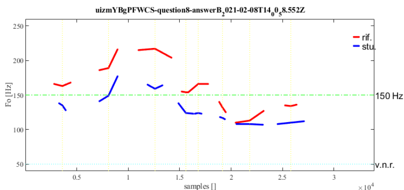
Figure 4 - Comparison of intonation curves between reference speaker (red) and user (blue) of the utterance “1/6 + 3/2”
