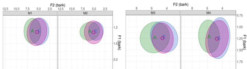
Figure 9 - Elicited speech vowel space for male couples
