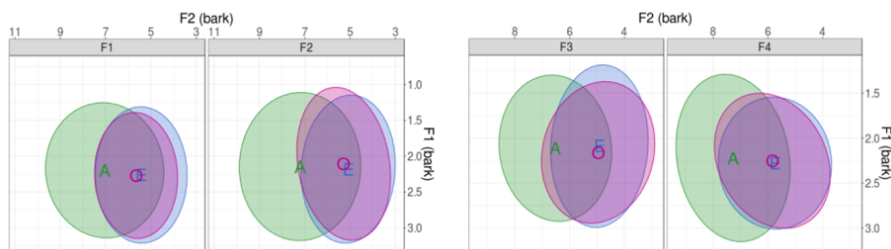
Figure 3 - Female couples' vowel space
